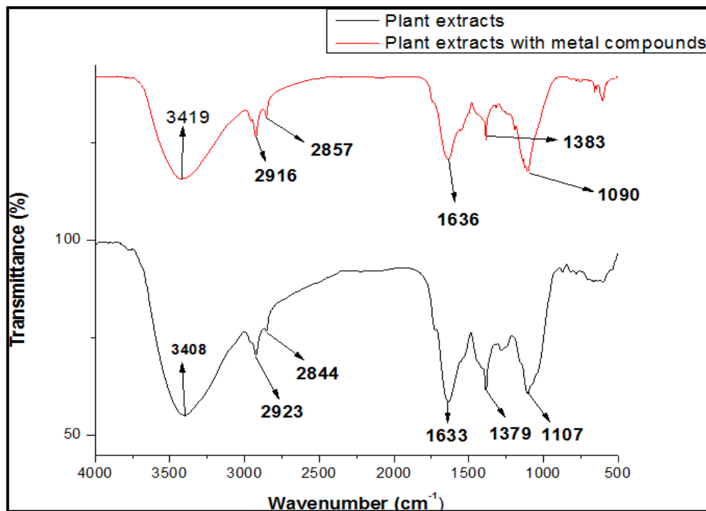
FIG 5. FT-IR spectrum of the synthesized Cu-NPs.
